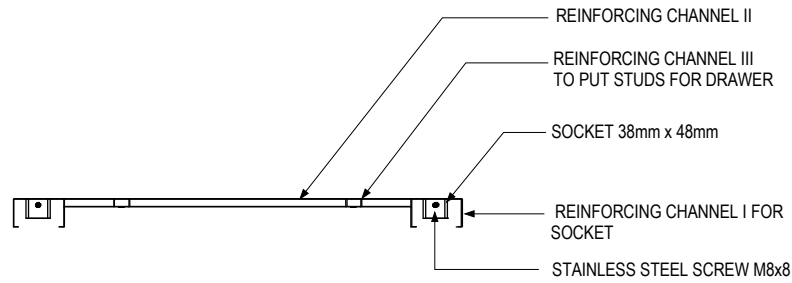
B CONSTRUCTION DETAILS
